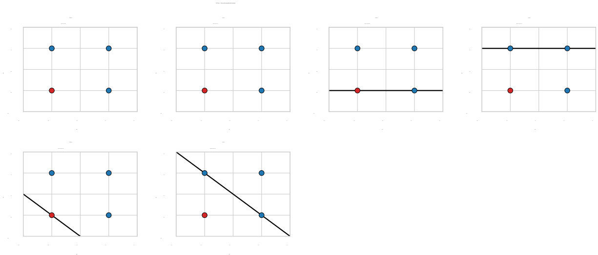
Figure 16: OR Gate – Decision Boundary After Each Update
