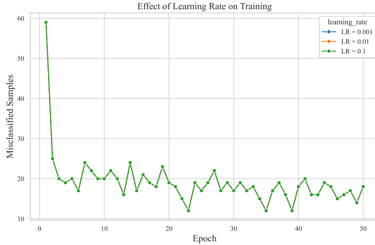
Figure 10: Learning Rate Comparison
