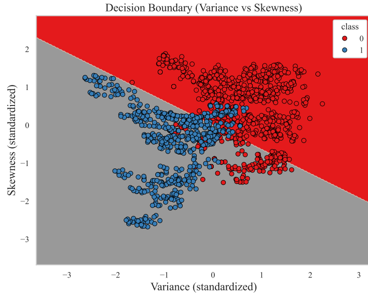
Figure 11: Decision Boundary using Variance and Skewness
