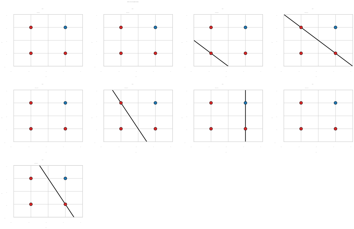
Figure 15: AND Gate – Decision Boundary After Each Update
